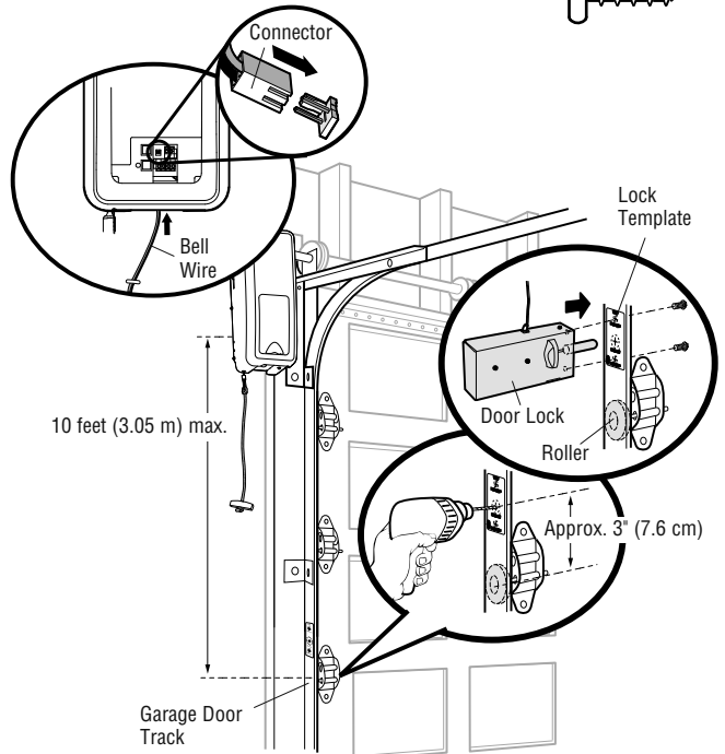
Screw 1/4"-20x1/2" (2)
